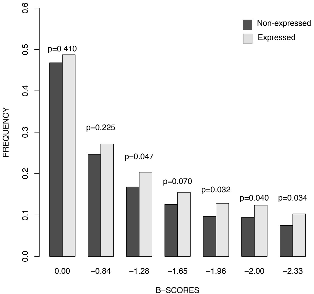
Supplemental Figure 2. Hits distribution across different B scores values. Distribution is evaluated for non-expressed (black bars) and expressed (light grey bars) sncRNAs in SH-SY5Y. We consider expressed miRNA as those showing above 1 count, according to the sequencing data.
