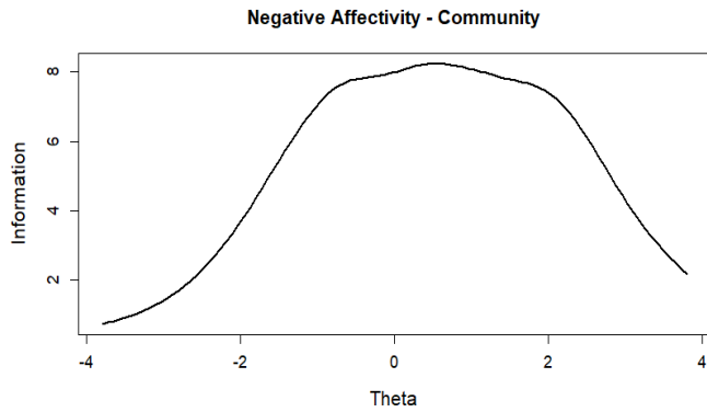
Figure S3. Test Information Curves from the PiCD and the SASPD in the Community (n = 2,522) and Clinical (n = 797) Samples.
