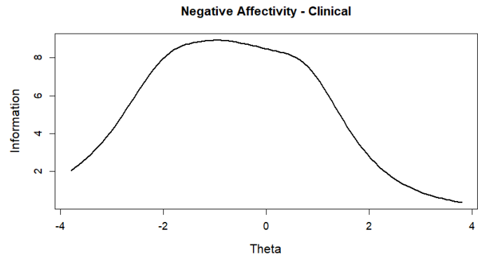
Figure S3. Test Information Curves from the PiCD and the SASPD in the Community (n = 2,522) and Clinical (n = 797) Samples.
