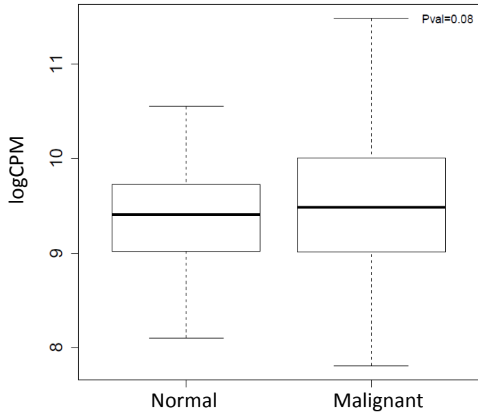
TCGA miRNA 374a-5p
