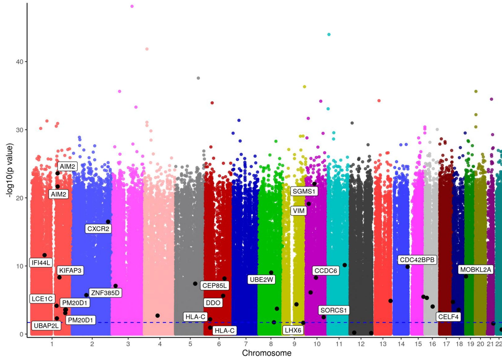
Supplementary Figure S2. Manhattan plot from the EWAS performed in the validation cohort. The plot shows the result of the COVID-19 severity association test over 735,349 CpG positions. The blue dashed line indicates the genome-wide significance threshold of a Benjamini-Hochberg corrected P value lower than 0.05. Black dots represent the 44 CpGs signature labeled with their corresponding genes.
