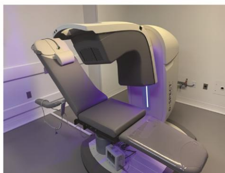
Figure 14 The D-SPECT is a CZT-system with nine rotating detector columns arranged over a stationary gantry (left). CZT-based cameras have the capability to reduce radiation dose and shorten imaging time. The D-SPECT system can also improve comfort by imaging patients while sitting (right).
